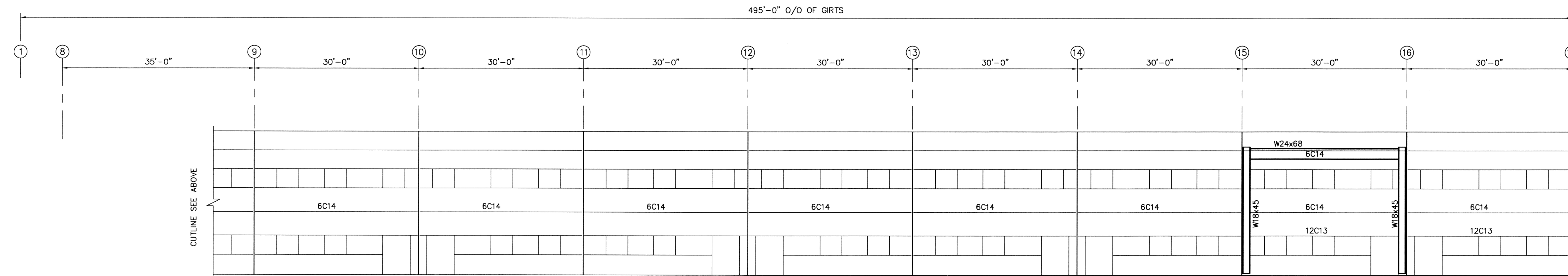
FRAMING ELEVATION @ LINE A ALL GIRTS TO BE 12C14 UNO ALL FRAMED OPENINGS TO BE 12C14
