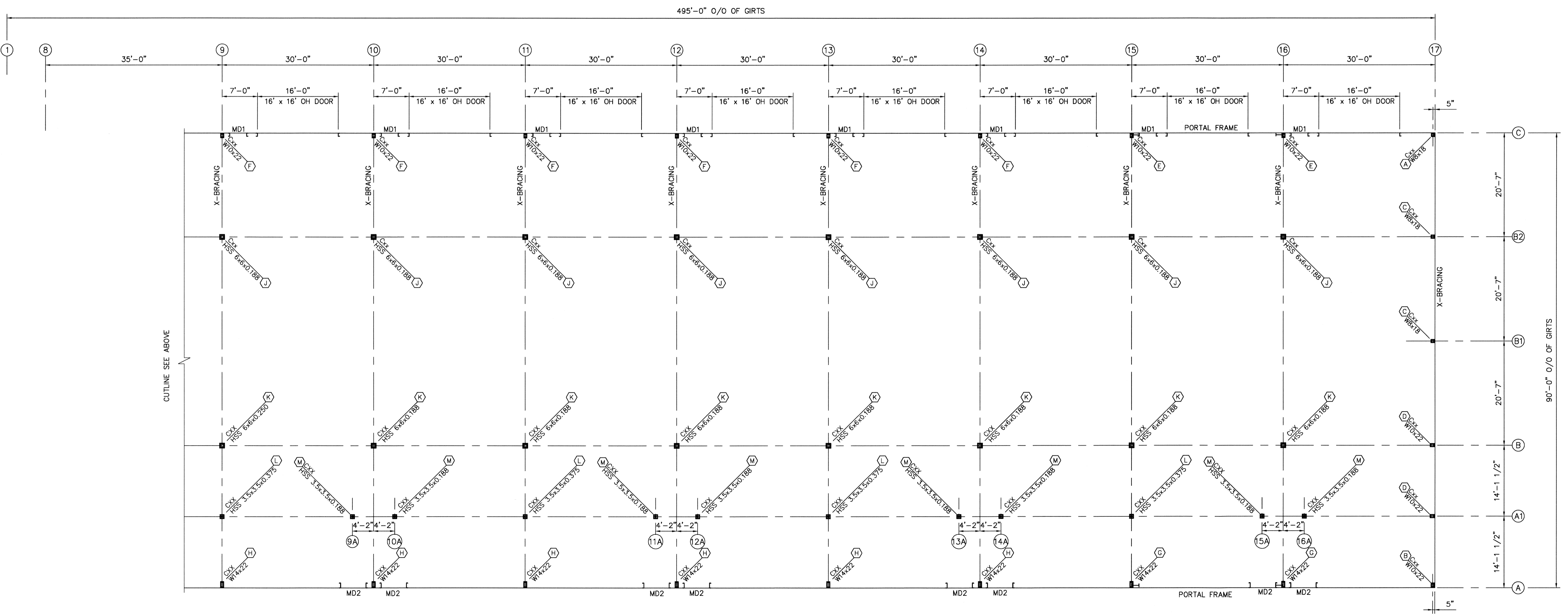
ANCHOR BOLT LAYOUT
